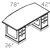
TOP-7842DPBT Bow Top Double Pedestal Desk W/Dictation Slide & Center Drawer
