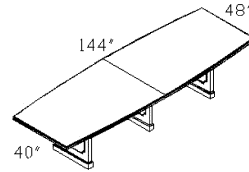
TOP-14448T 2" Top Boat Shape Conference Table (Two Sections)
