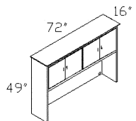
TOP-7216H Hutch W/Wood Doors
