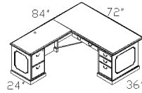
TOP-EL L/R 'L' W/72" Desk – Left or Right W/Center Drawer
