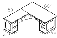
TOP-EL6630 L/R 'L' W/66" Desk – Left or Right W/Center Drawer
