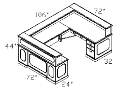
TOP-RUU L/R Reception 'U' Unit – Left or Right W/Center Drawer & Keyboard Slide
