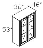
TOP-3616GH Bookcase W/Glass Doors (Specify Free Standing/Stacking)
