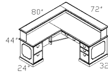
TOP-RUL L/R Reception 'L' Unit – Left or Right W/Center Drawer
